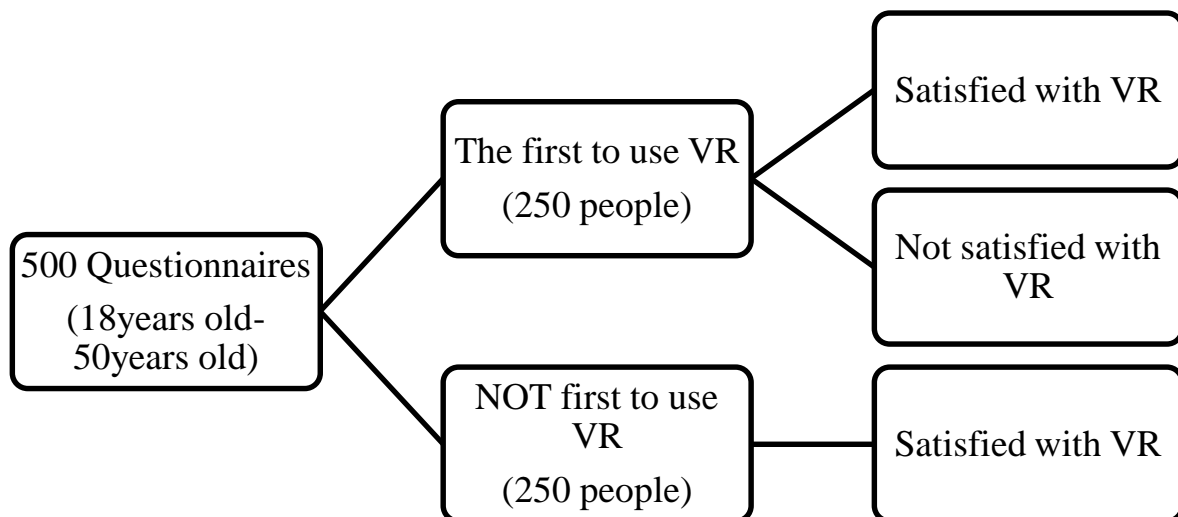
Figure 6. Conceptual framework
